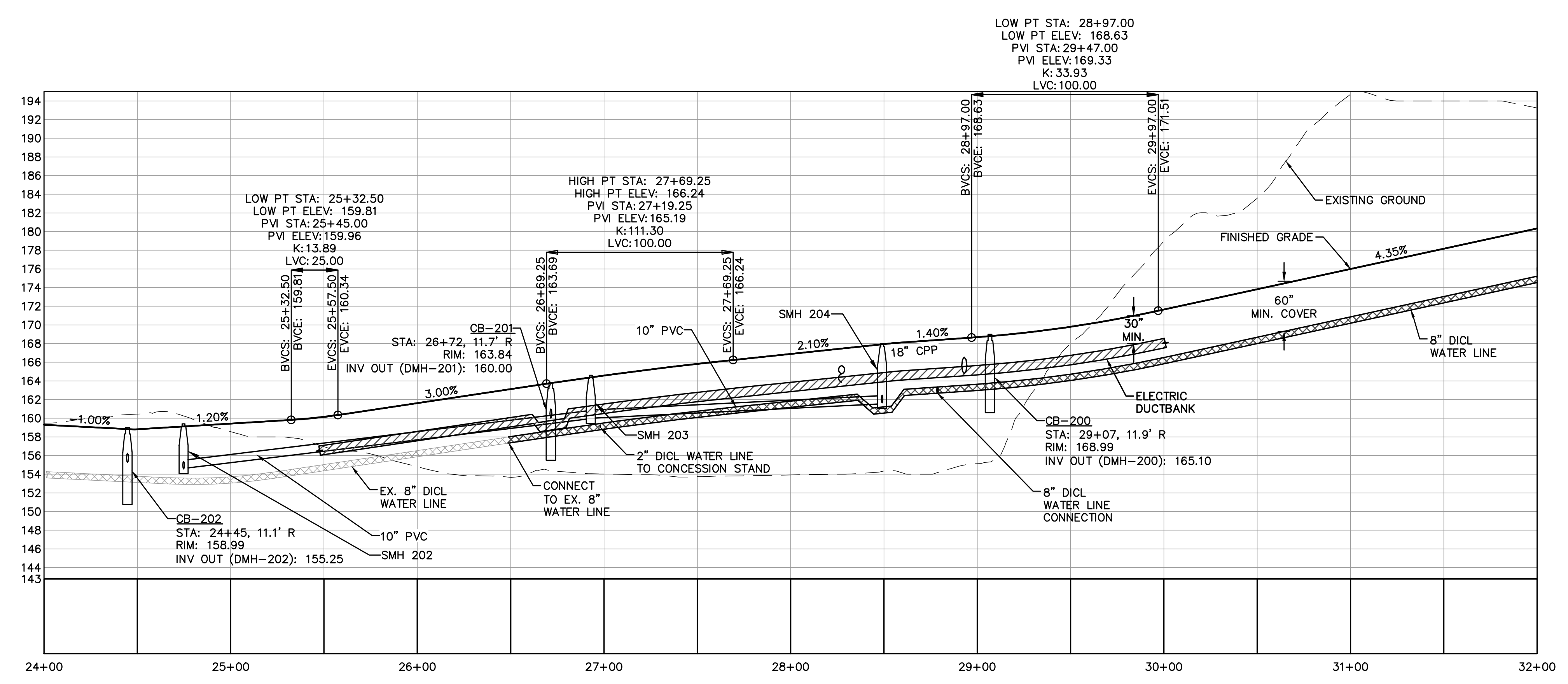
DRIVEWAY LOOP PROFILE STA 24+00 TO STA 32+00
