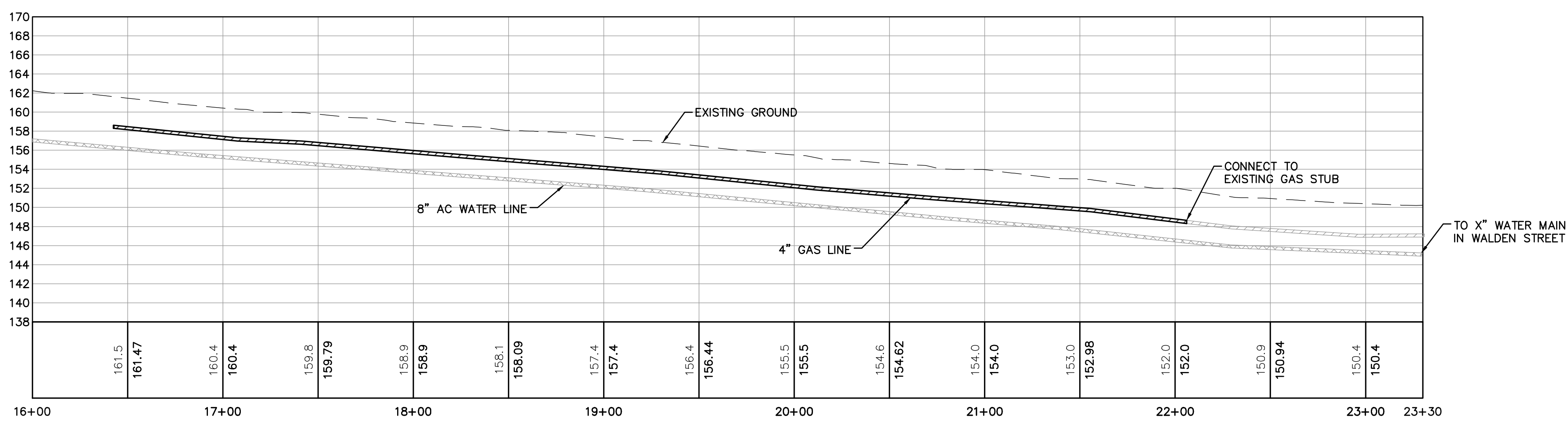
FRONT DRIVEWAY PROFILE STA 16+00 TO STA 23+30
