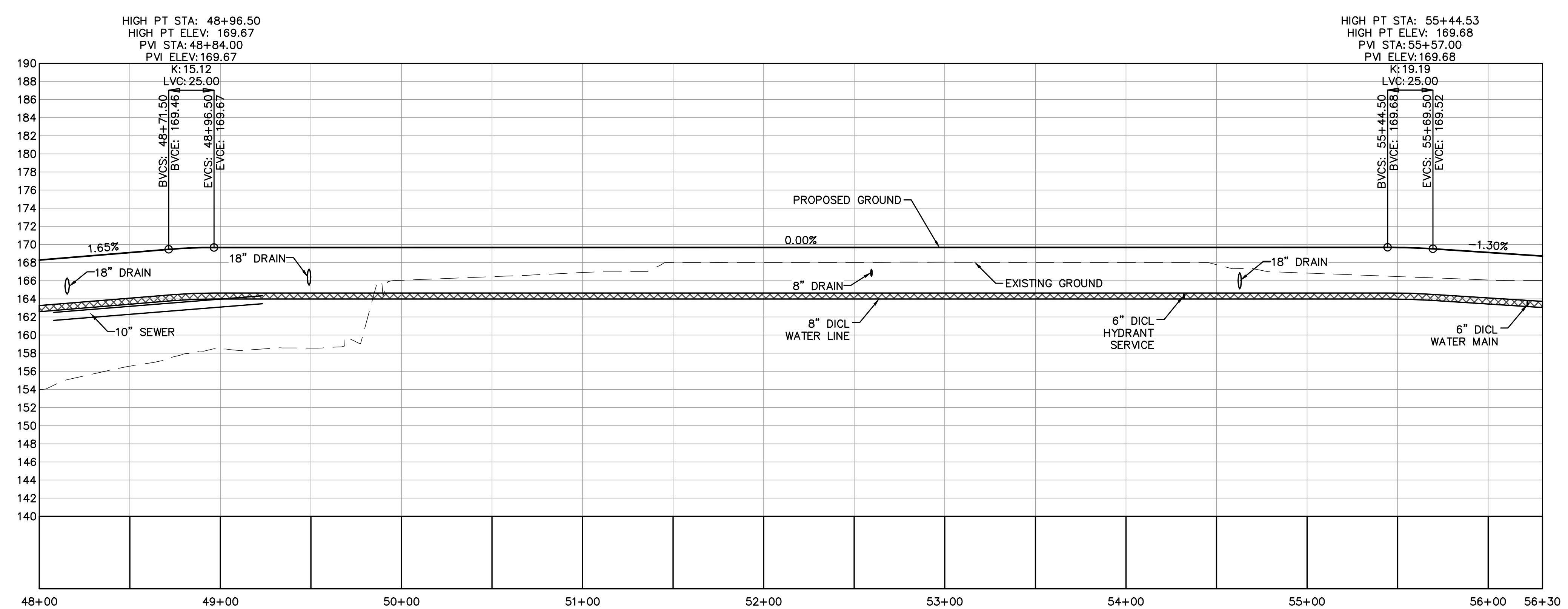
CENTER DRIVEWAY PROFILE STA 48+00 TO STA 56+30
