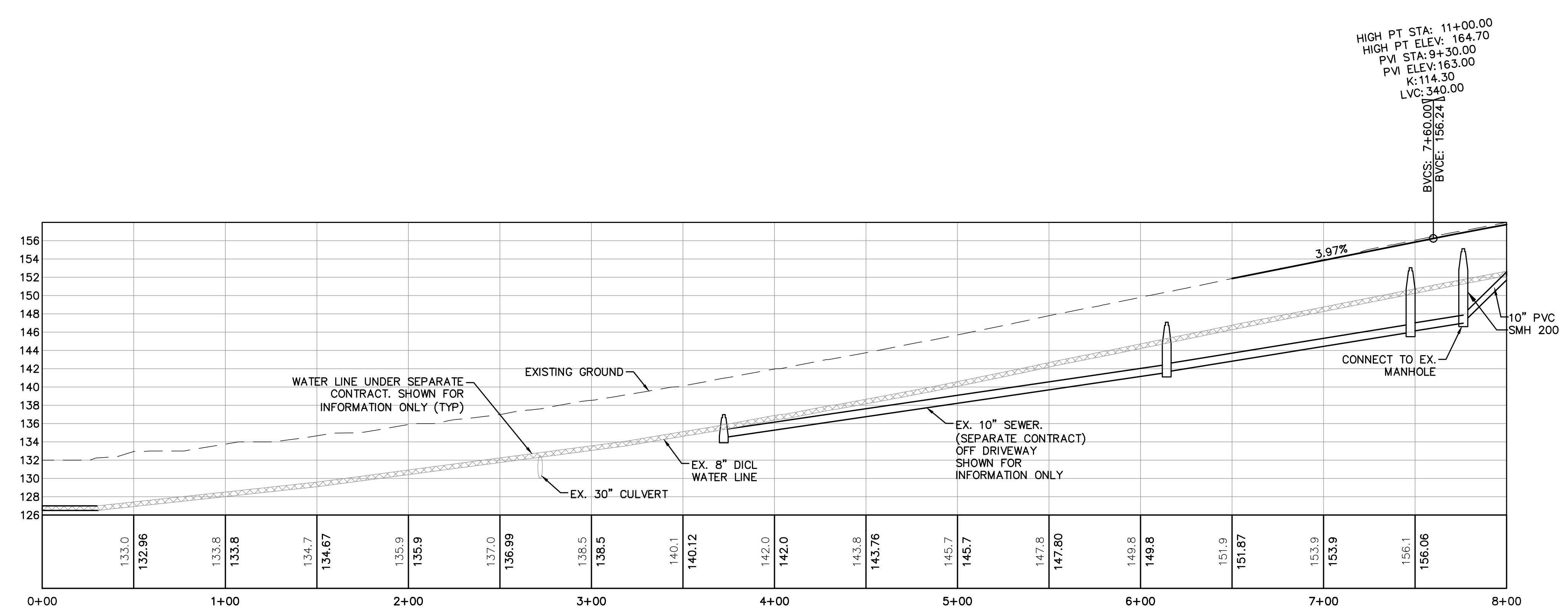
FRONT DRIVEWAY PROFILE STA 0+00 TO STA 8+00
