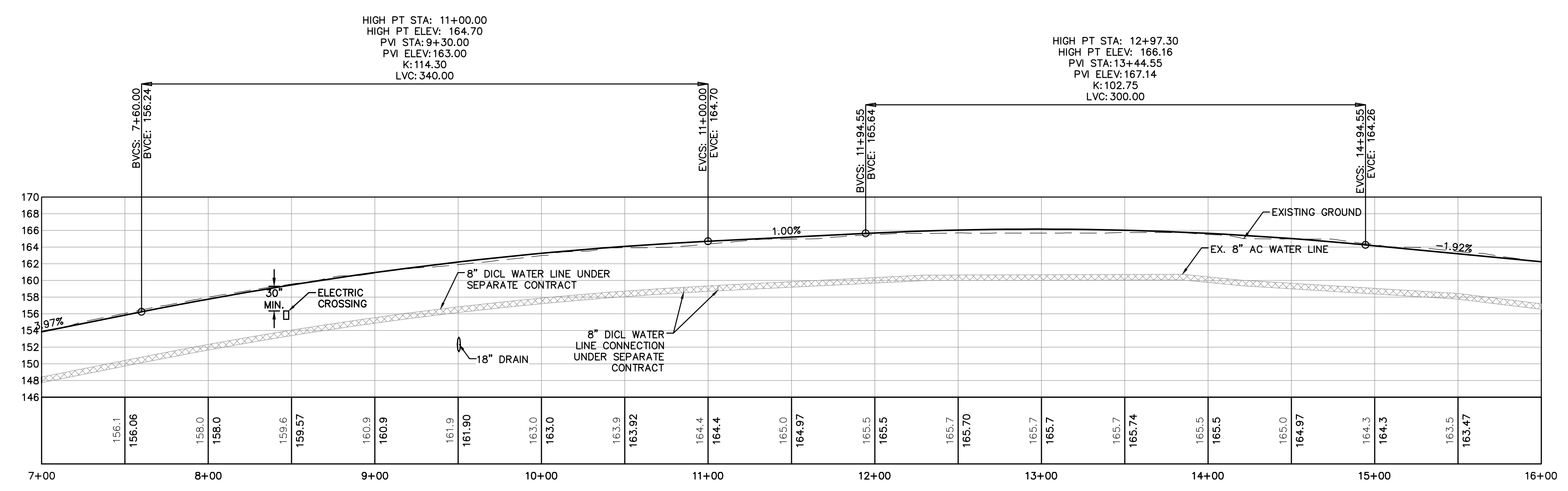
FRONT DRIVEWAY PROFILE STA 7+00 TO 16+00
