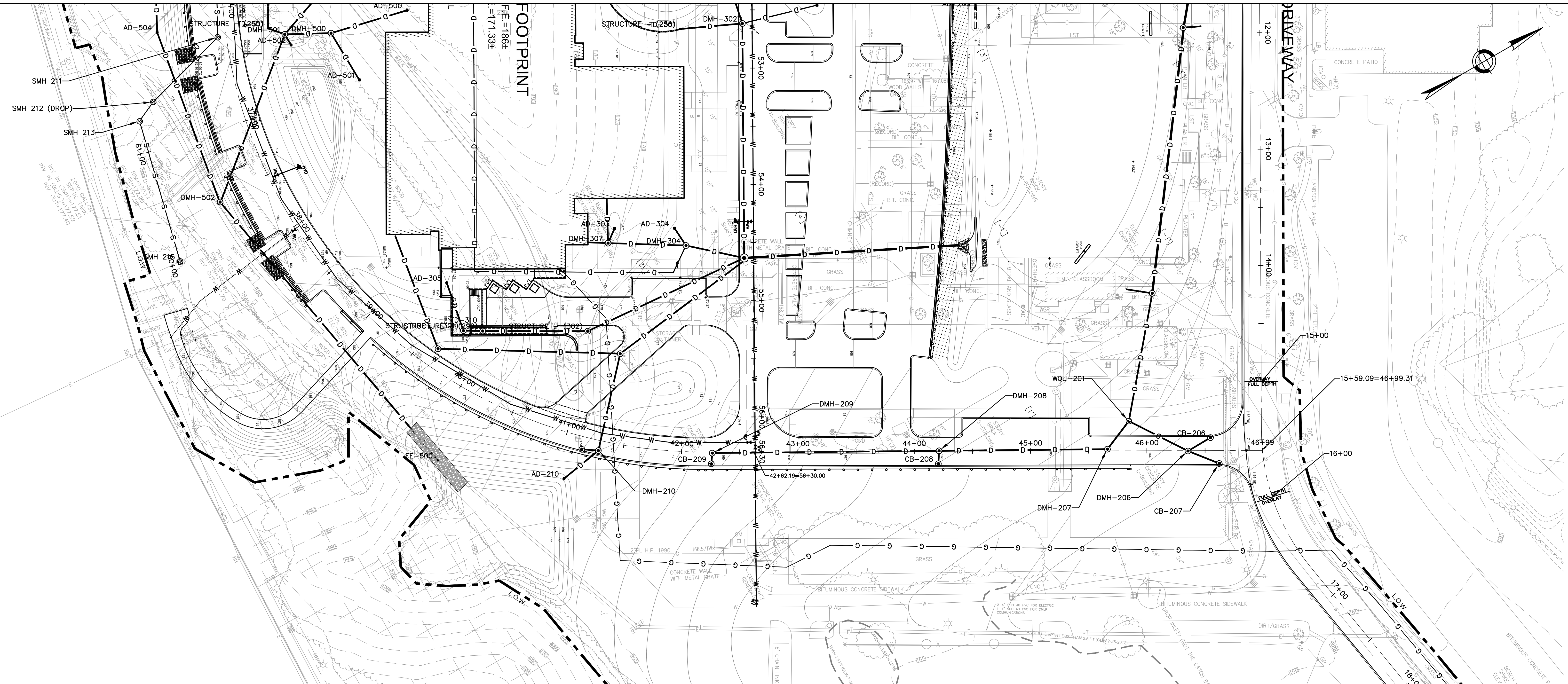
PLAN VIEW
